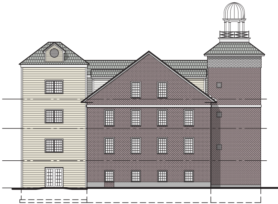
4 SOUTH ELEVATION RHS
