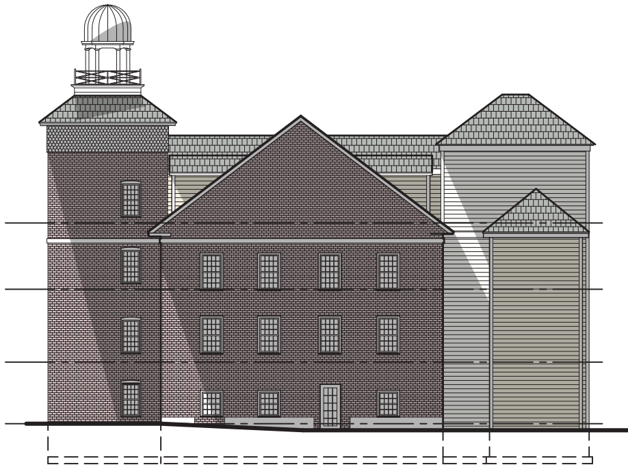
2 NORTH ELEVATION RHS
