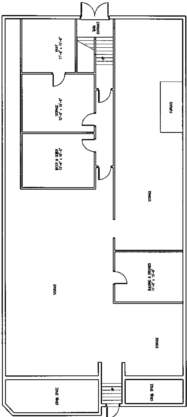
BASEMENT PLAN
