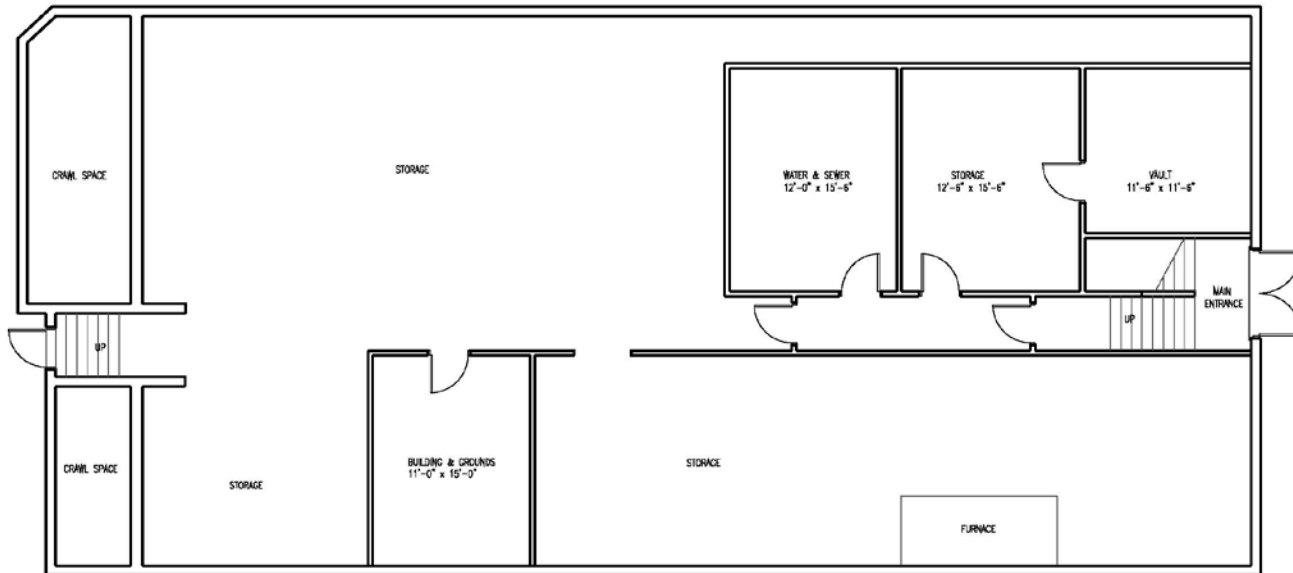
BASEMENT PLAN
